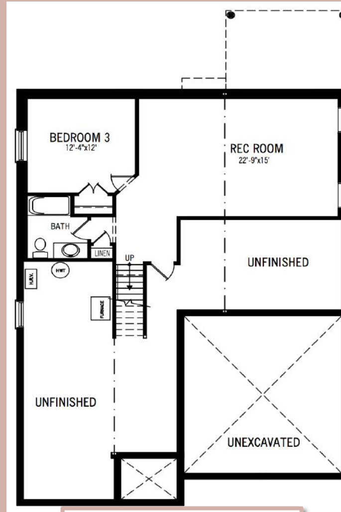
BASEMENT PLAN
