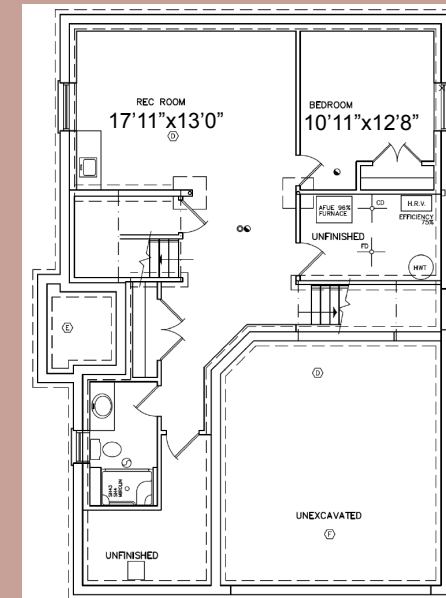
BASEMENT PLAN
